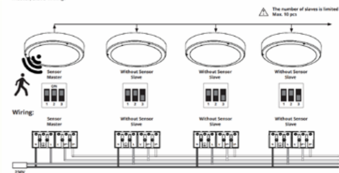
Master/Slave Wiring:
